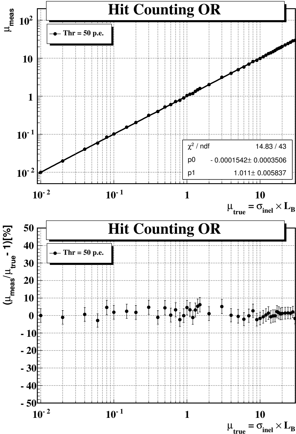
Figure 51. Top: average number of pp interactions per event measured ( \mu_{meas} ) with the polynomial fit model with hit counting “OR” method versus the true value ( \mu_{true} ). A linear fit is superimposed. Bottom: deviation from the true value.
