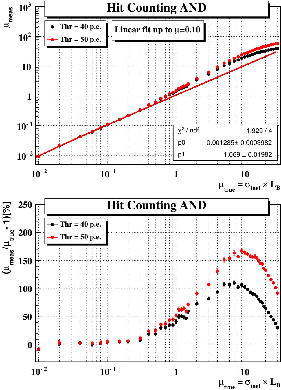
Figure 44. Top: average number of pp interactions per event measured with a linear extrapolation of N_{\text{hits}/BX}^{\text{AND}} from \mu = 0.01 for two different thresholds (40 and 50 p.e.). Bottom: deviation from the true value.
