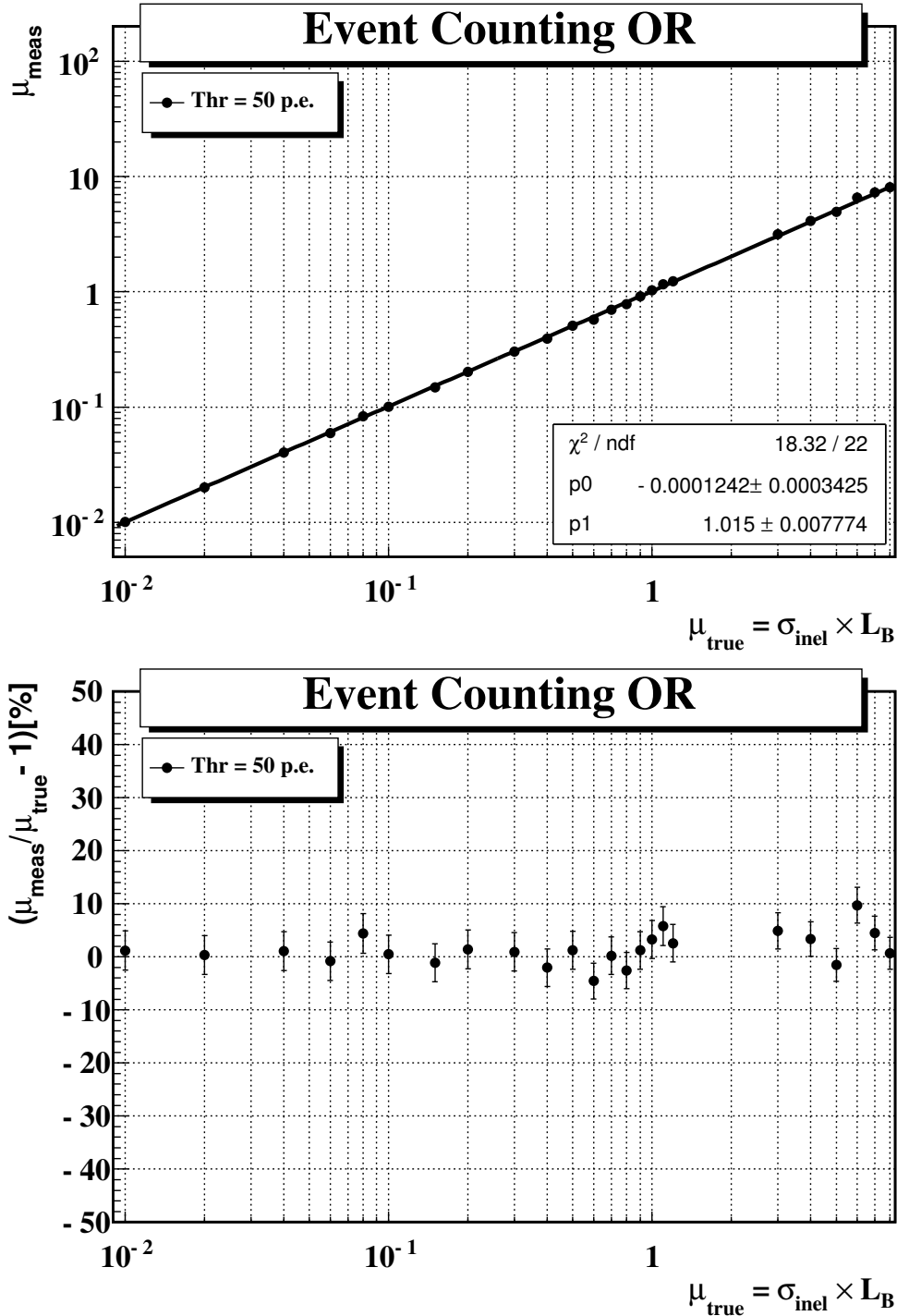
Figure 47. Top: average number of pp interactions per event measured with the polynomial fit model by using the event counting “OR” method versus the true value. A linear fit is superimposed. Bottom: deviation from the true value.
