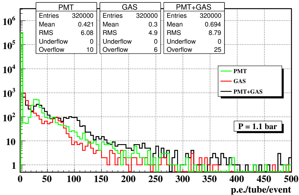
Figure 9. Photo-electrons detected by LUCID in 10000 events of single pions coming from the IP with E = 180 GeV and a random direction ( 0.004 < \theta < 0.01 , 0 < \phi < 2\pi ).
