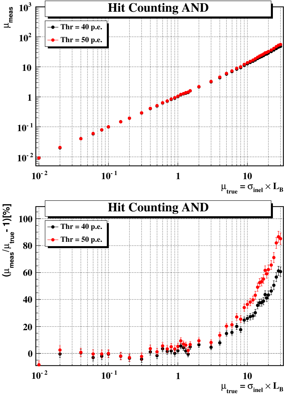
Figure 43. Top: average number of pp interactions per event measured with the hit counting “AND” method as a function of the true value for two different thresholds (40 and 50 p.e.). Bottom: deviation from the true value.
