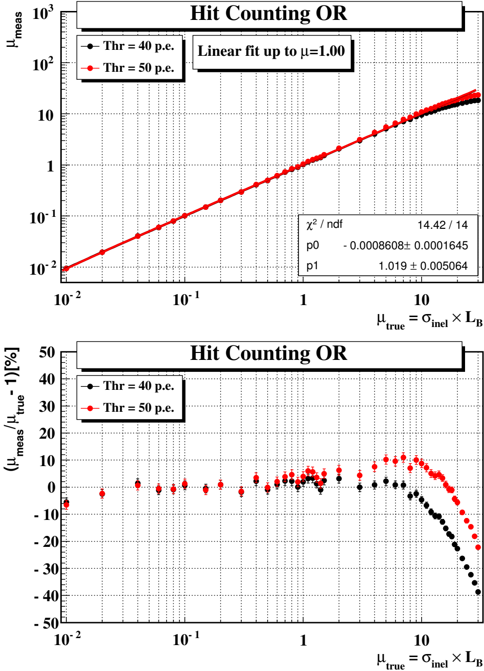
Figure 42. Top: average number of pp interactions per event measured with a linear extrapolation of N_{\text{hits}/BX}^{\text{OR}} from \mu = 0.01 for two different thresholds (40 and 50 p.e.). Bottom: deviation from the true value.
