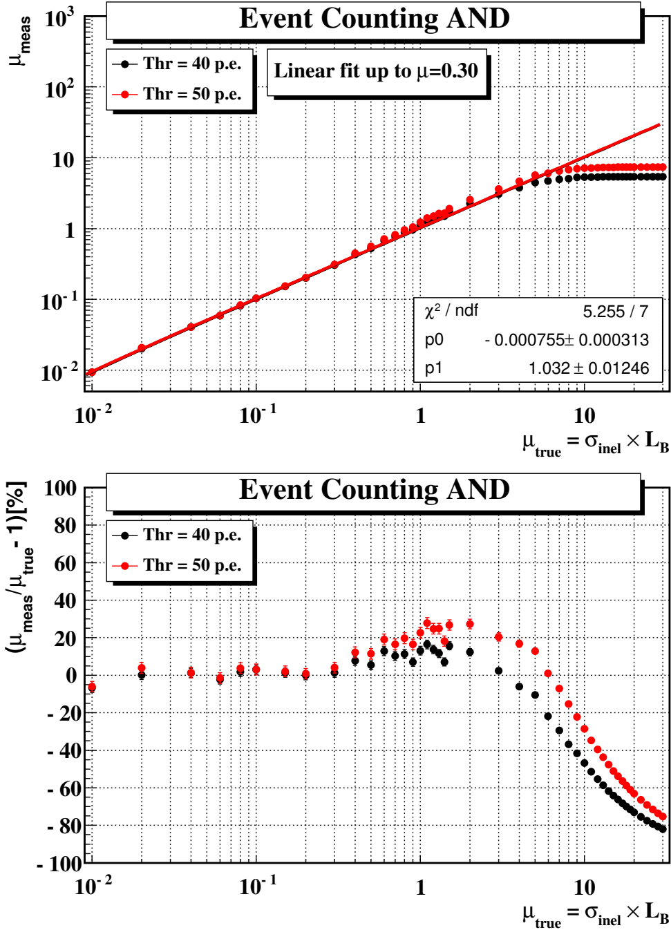
Figure 40. Top: average number of pp interactions per event measured with a linear extrapolation of P_{\text{hits}/BX}^{\text{AND}} from \mu = 0.01 for two different thresholds (40 and 50 p.e.). Bottom: deviation from the true value.
