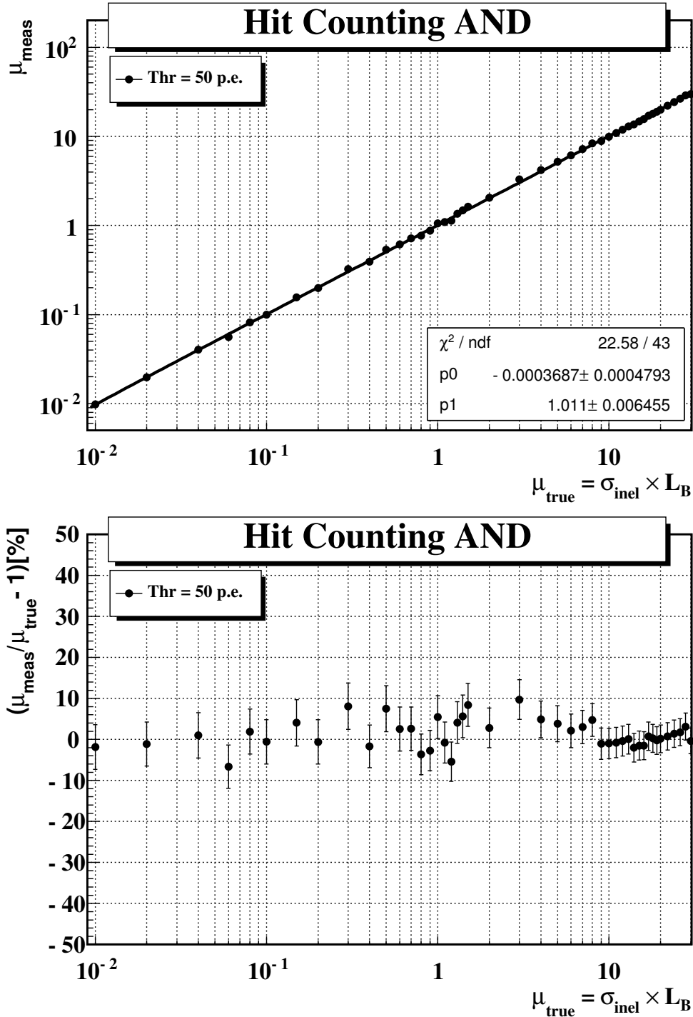
Figure 52. Top: average number of pp interactions per event measured ( \mu_{meas} ) with the polynomial fit model with hit counting “AND” method versus the true value ( \mu_{true} ). A linear fit is superimposed. Bottom: deviation from the true value.
