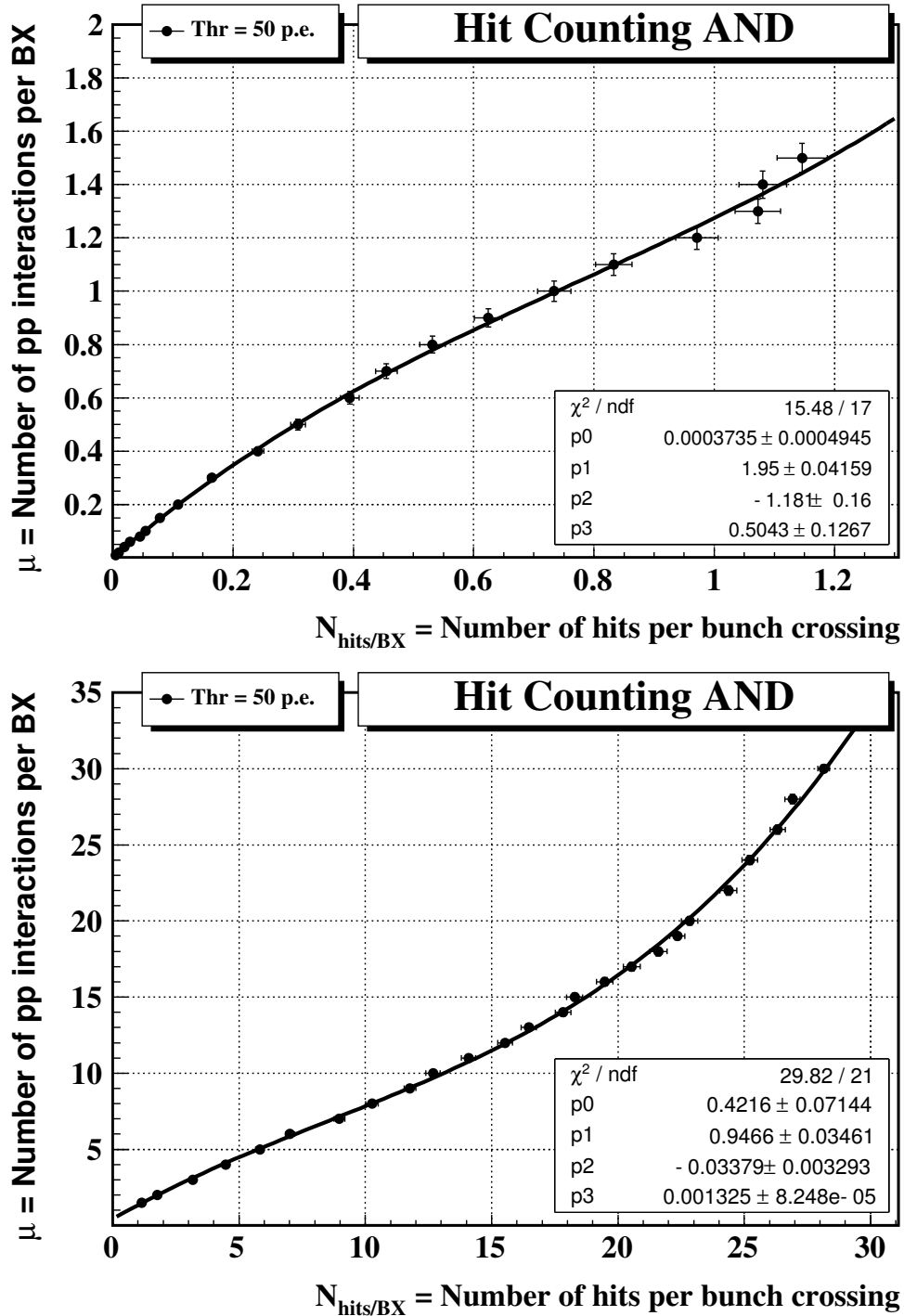
Figure 50. Average number of pp interactions per event ( \mu ) as a function of the average number of hits per event ( N_{\text{hits/BX}} ) with hit counting “AND” method. The distribution is fitted with a 4th degree polynomial for \mu < 1.2 (top) and \mu > 1.2 (bottom).
