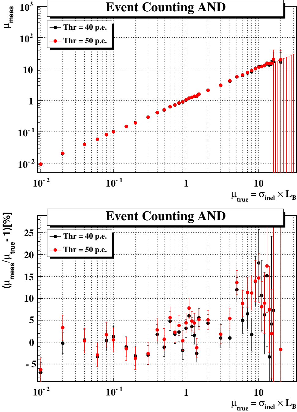
Figure 39. Top: average number of pp interactions per event measured with the event counting “AND” method as a function of the true value for two different thresholds (40 and 50 p.e.). The logarithmic correction given by the combinatorial model is included. Bottom: deviation from the true value.
