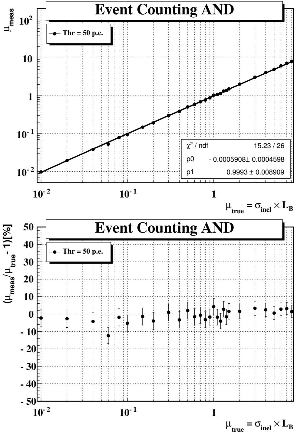
Figure 48. Top: average number of pp interactions per event measured with the polynomial fit model by using the event counting “AND” method versus the true value. A linear fit is superimposed. Bottom: deviation from the true value.
