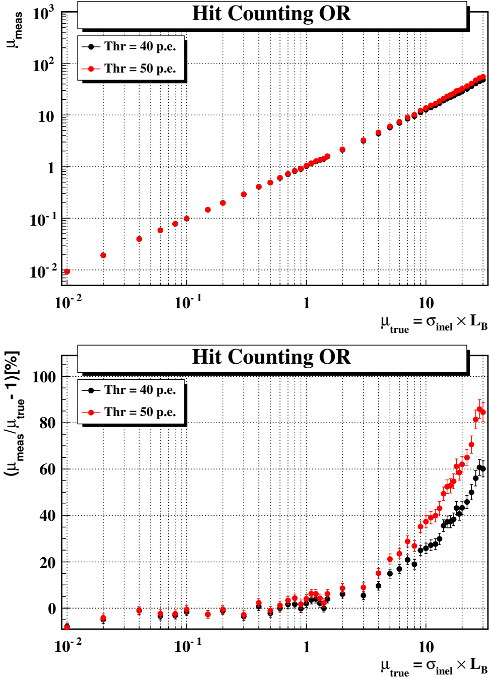
Figure 41. Top: average number of pp interactions per event measured with the hit counting “OR” method as a function of the true value for two different thresholds (40 and 50 p.e.). Bottom: deviation from the true value.
