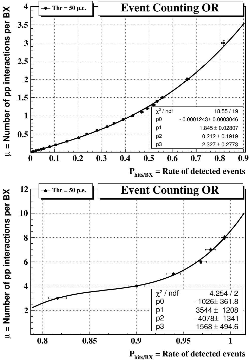
Figure 45. Polynomial fits of the average number of pp interactions per event ( \mu ) as a function of the average number of detected events ( P_{hits/BX} ) with event counting “OR” method for P_{hits/BX} < 0.8 (top) for P_{hits/BX} > 0.8 (bottom).
