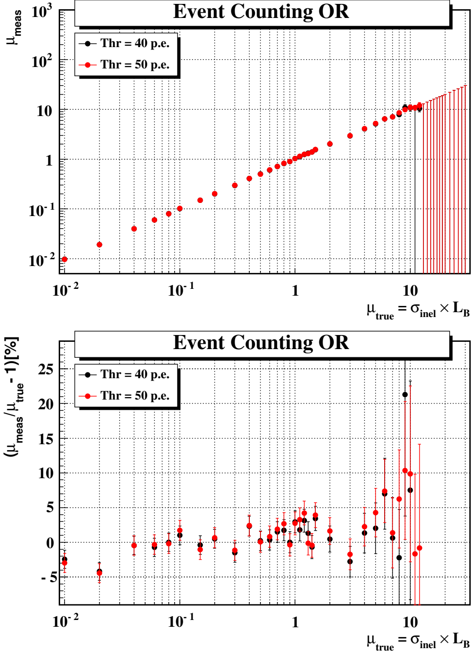
Figure 37. Top: average number of pp interactions per event measured with the event counting “OR” method as a function of the true value for two different thresholds (40 and 50 p.e.). The logarithmic correction given by the combinatorial model is included. Bottom: deviation from the true value.
