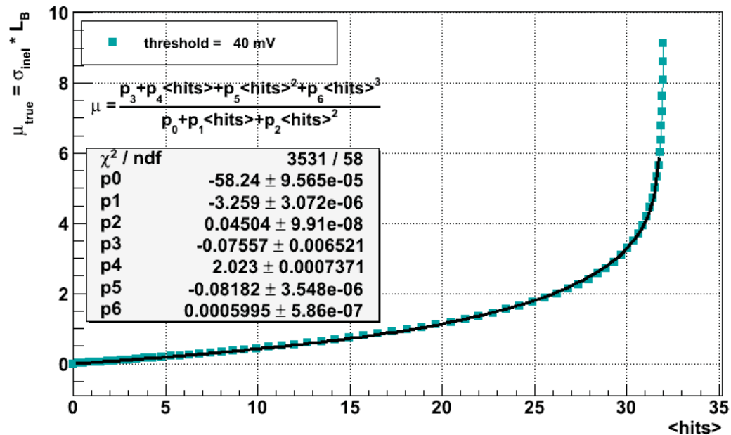
Hits Counting - AND, PYTHIA NON DIFF. 10 TeV
