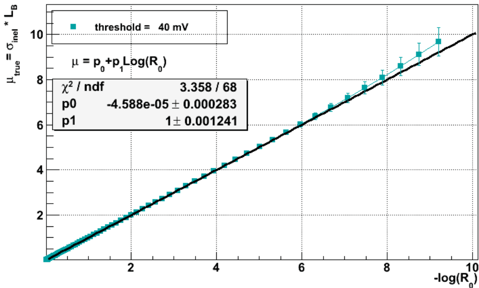
Zero Counting - OR, PYTHIA NON DIFF. 10 TeV
