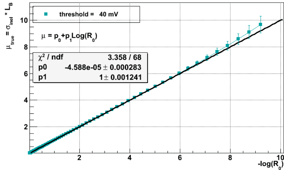
Zero Counting - AND, PYTHIA NON DIFF. 10 TeV
