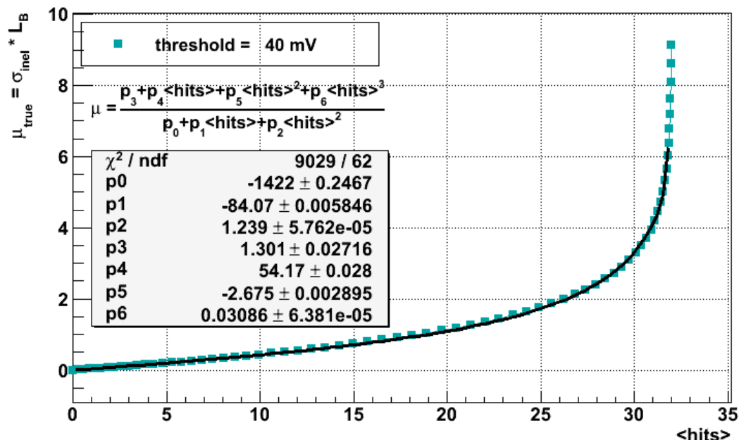
Hits Counting - OR, PYTHIA NON DIFF. 10 TeV
